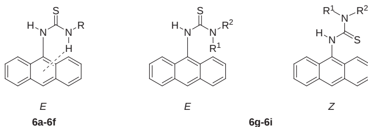
FIG. 2 Conformations of thioureas 6a–6i
