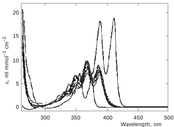
FIG. 3 UV-VIS spectra of anthracene, 9-isothiocyanatoanthracene ( 5 ) and 1-alkyl-(3-anthracene-9-yl)-thioureas 6a–6h
